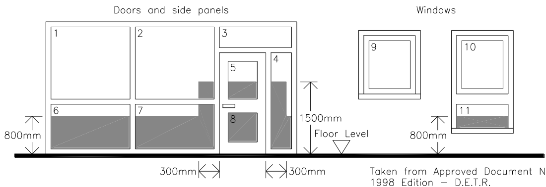
Diagram 1 Critical locations in internal and external walls
