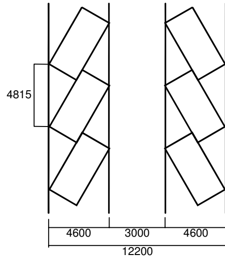
30° Approach Angle
