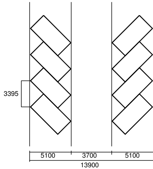
45° Approach Angle
