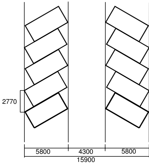
60° Approach Angle
